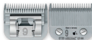
GT333 2,0 mm
